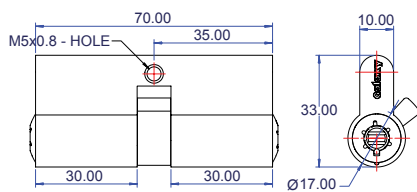
Floating Cam version
