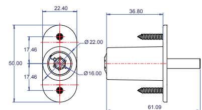
Pushlock
