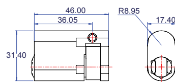
Union Single (Oval)
