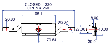
Garage Door Lock
