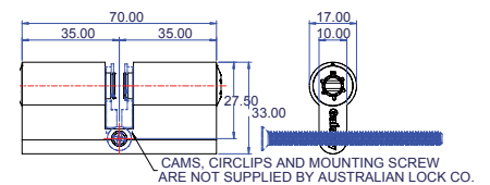
Gainsborough TriLock
