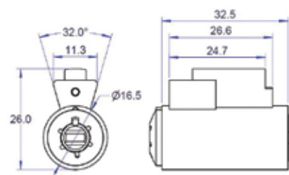
Lockwood 500 V7
