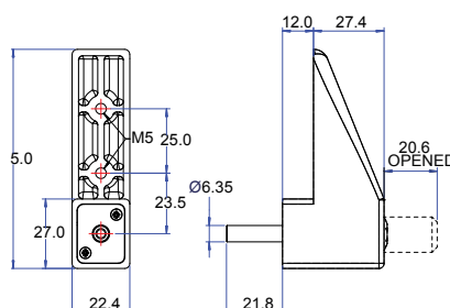
Showcase Lock
