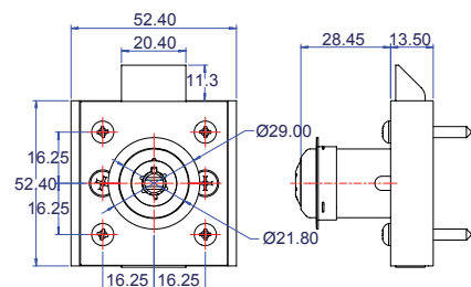
Aluminium Cupboard/Drawer Lock Standard - Latching
