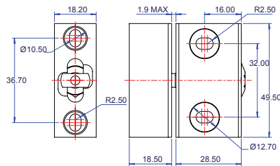
Fridge Lock
