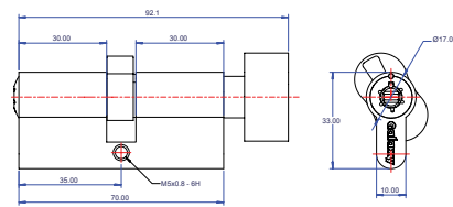
Floating Cam version
