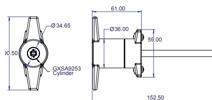
Tee Handle
