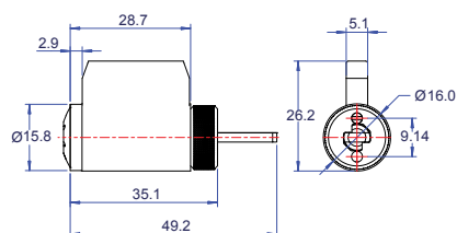
Boyd B162P, 12Z, B462P, B862P & Schlage
