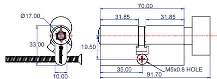
Thumbturn Euro Profile - Fixed Cam
