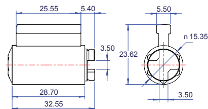
Lockwood 530
