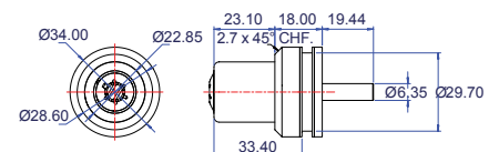
Thru-Glass Pushlock
