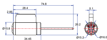
Boyd D&H Series - (Long Tail) Schlage
