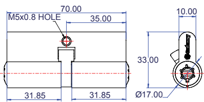
Euro Profile Double - Fixed Cam
