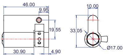
Euro Profile Single Cylinder
