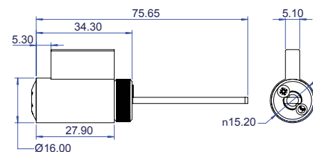
Whitco W5000
